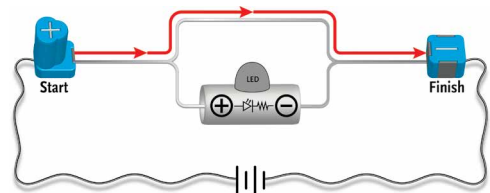
Beacon in parallel with bypass metal strip – Beacon does not light
